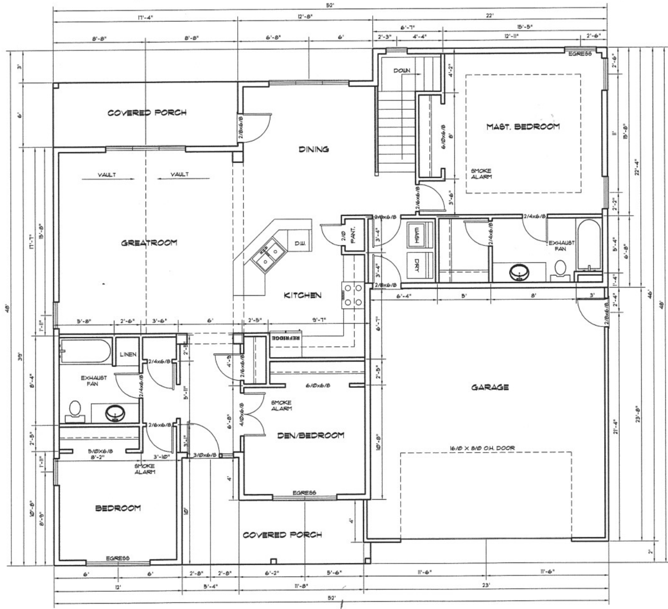
FLOOR PLAN 1600 SQ. FT. SCALE: 1/4" = 1'-0"
